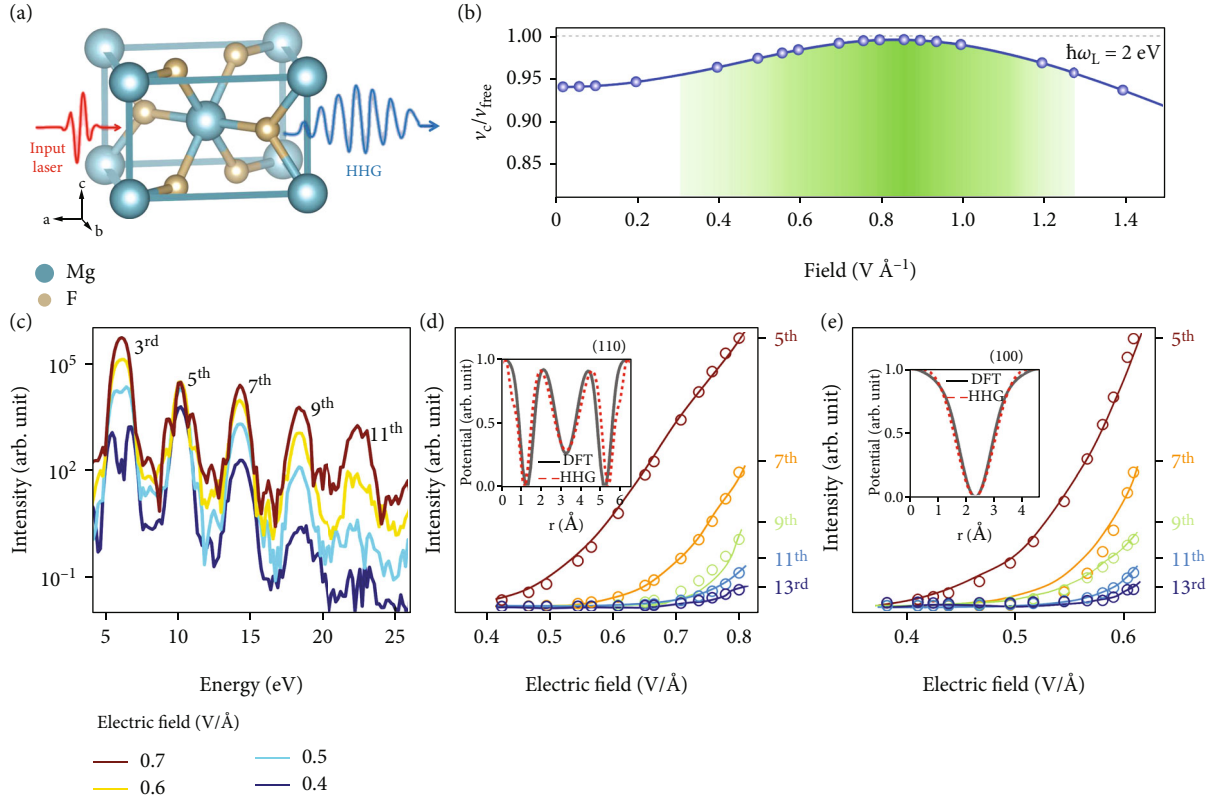
FIGURE 3: The reconstructed valence electron potential of MgF 2 via HHG spectra. (a) Schematics showing the high order harmonic generation in solid MgF 2 . (b) Ratio of the maximum of crystal ( v_c(t) ) and free ( v_{free}(t) ) electron velocities along [100] direction of MgF 2 crystal as a function of field strength of the driving pulse with a carrier photon energy of 2 eV. (c) The HHG spectrum with electric field polarization along [110] direction. The HHG intensity as a function of electric field strength along [110] (d) and [100] (e) directions. The cycle symbols are the data points and the solid lines are the fitting lines. The insets in (d) and (e) show the valence electron potential distribution along [110] and [100] directions. The solid black and dashed red lines label the potential obtained by the DFT calculation and HHG spectrum reconstruction, respectively.
