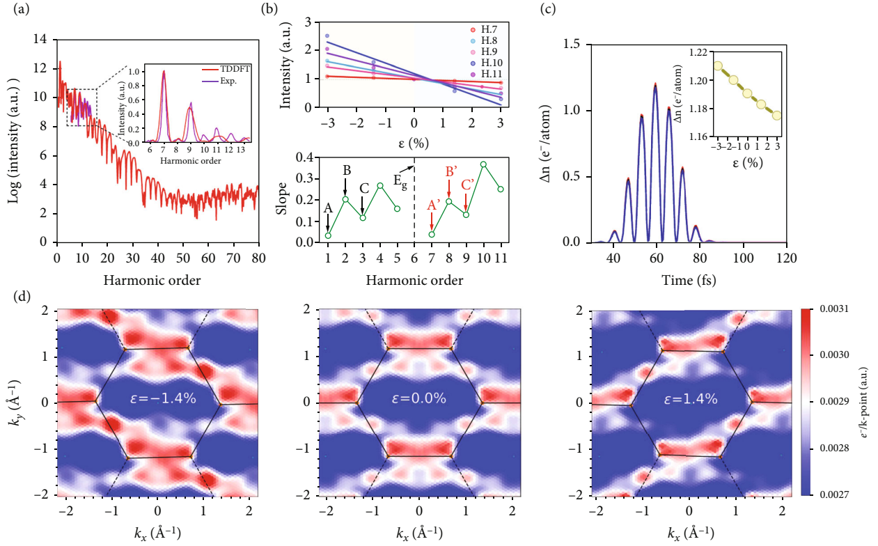
FIGURE 4: Electronic excitation mechanisms in strained 1 L-MoS 2 . (a) HHG spectrum of primitive 1 L-MoS 2 from TDDFT calculation (red) and its comparison with the experimental measurement (purple). (b) Dependence of HHG intensity on the applied strain, and the absolute values of slope corresponding to representative harmonics. (c) Number of electrons excited to the conduction bands during the laser illumination. The inset shows the maximum value of excited electrons ( t = 60 fs) as a function of strain. (d) Distribution of the photoexcited electrons in Brillouin zone at t = 60 fs under three strain conditions.
