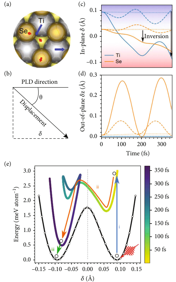
FIGURE 7: Photoexcited lattice dynamics in TiSe 2 . (a) The nontrivial symmetrically inequivalent Ti and Se atoms with PLD. (b) Schematic diagram of in-plane displacement \delta . (c, d) The in-plane and out-of-plane displacement \delta , \delta_z , respectively. (e) The curve marked by hollow circles and the other curve indicate the ground state potential energy surface (PES) and the nonequilibrium time-dependent PES, respectively.
